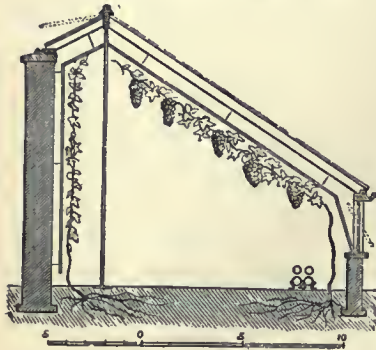
FIG. 6.—Hip-Roofed Vinery.
